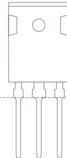
TO-247AD MTO-3P,3PT,3PV
